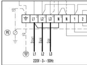
220V 50Hz tri-phase wiring
